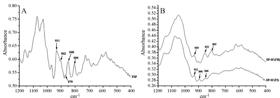
Fig. 2. Infra red spectra (400–1200 cm −1 ) of S. filiformis . (A) Total sulfated polysaccharides (TSP). (B) Fractions SP-Sf (F I and F II).
